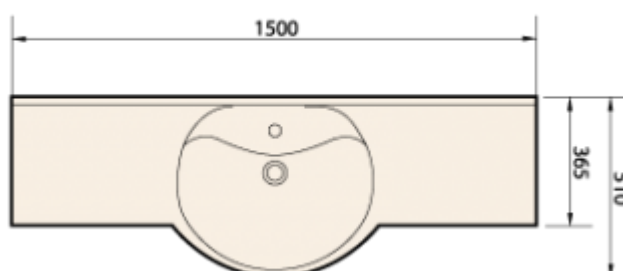
LAUDA 1500
