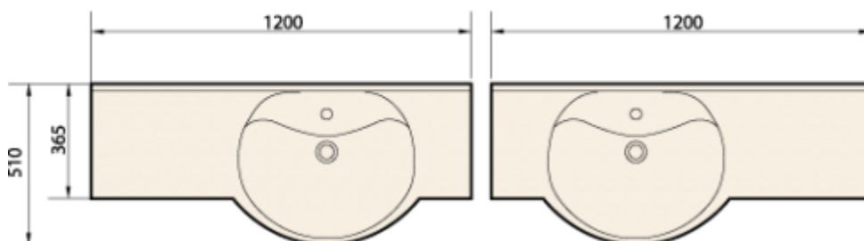
LAUDA 1200
